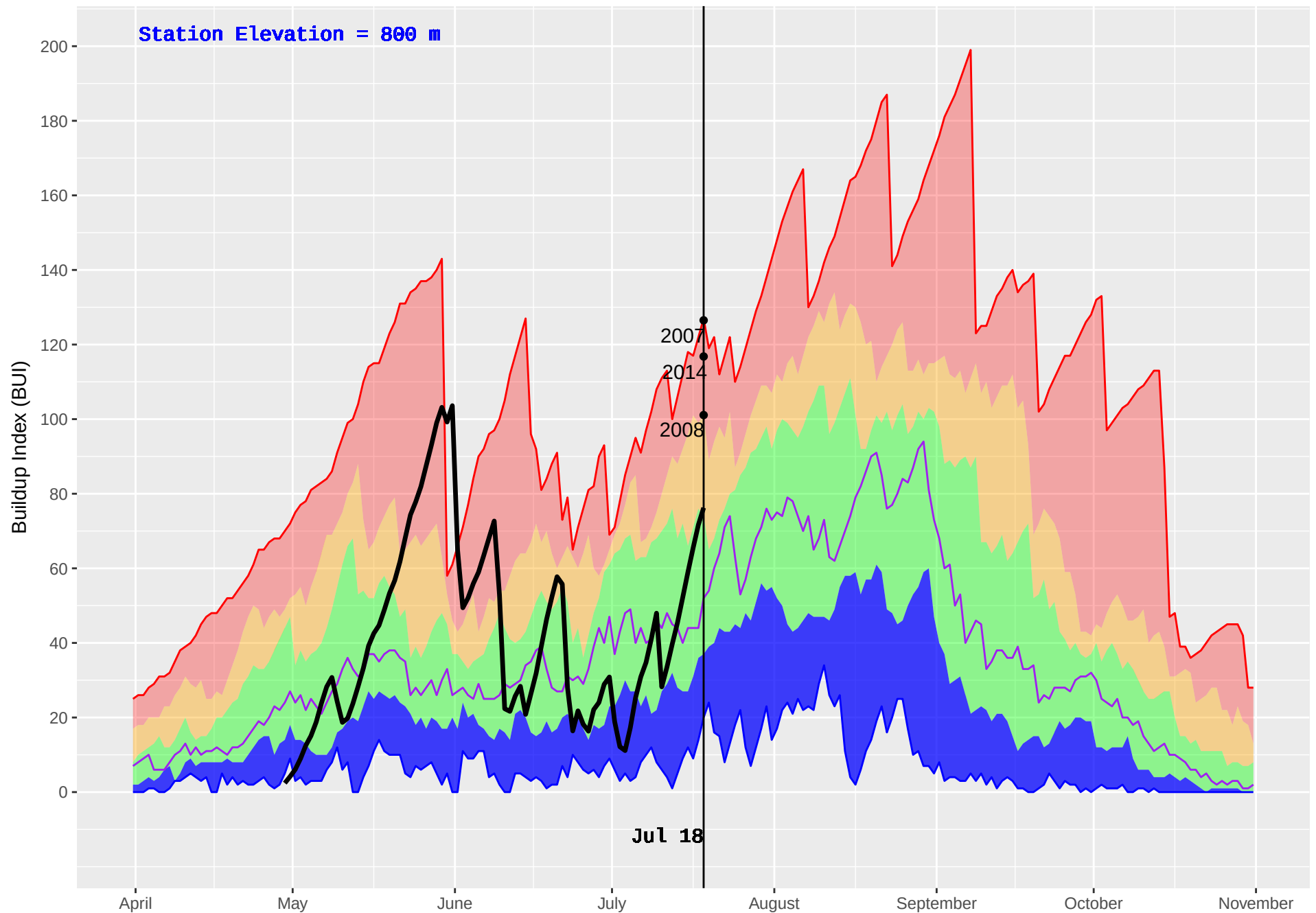
GOLD HILL (379) : Historical (1979–2016) and Current (2018) Daily Buildup Index (BUI)
