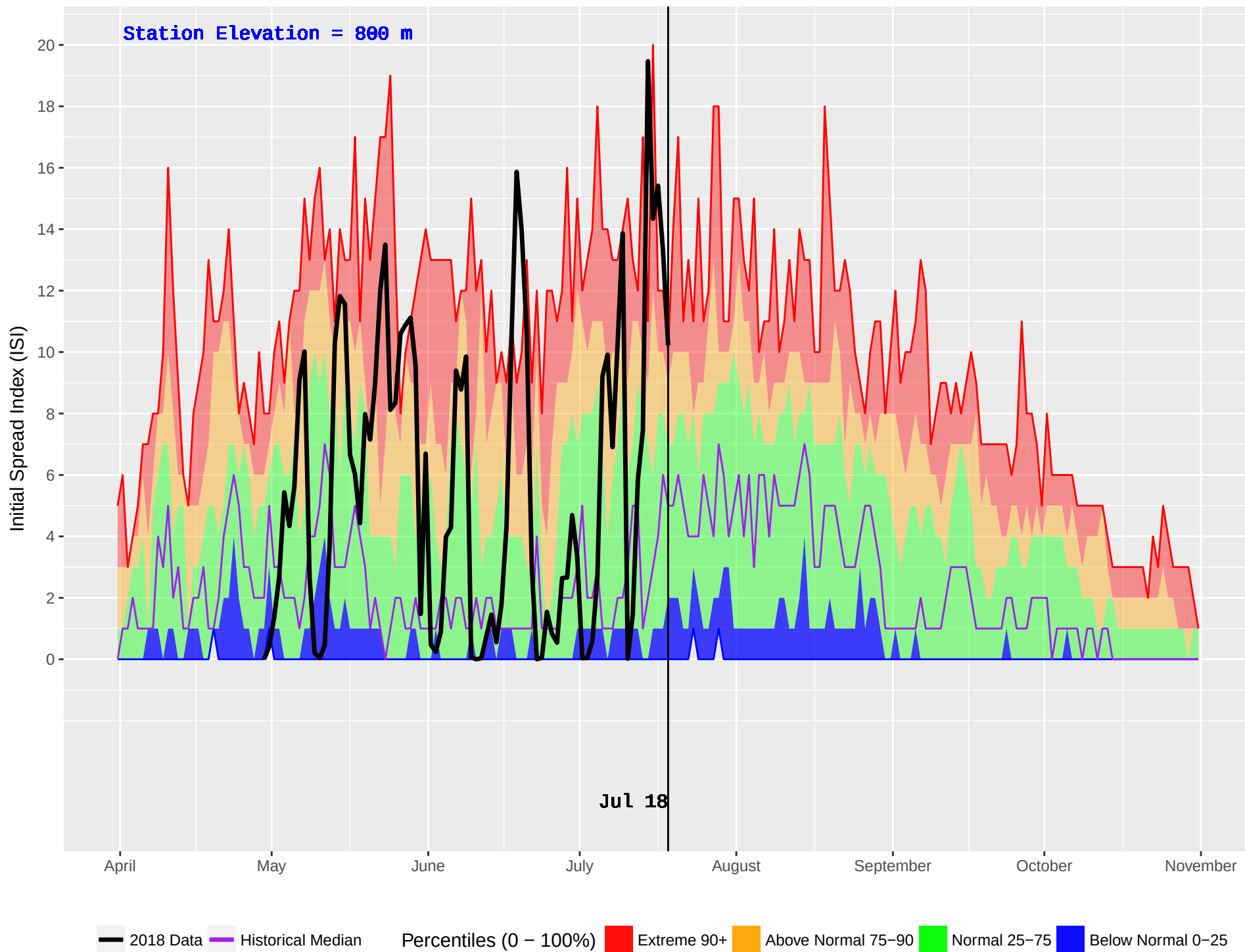
GOLD HILL (379) : Historical (1979–2016) and Current (2018) Daily Initial Spread Index (ISI)
