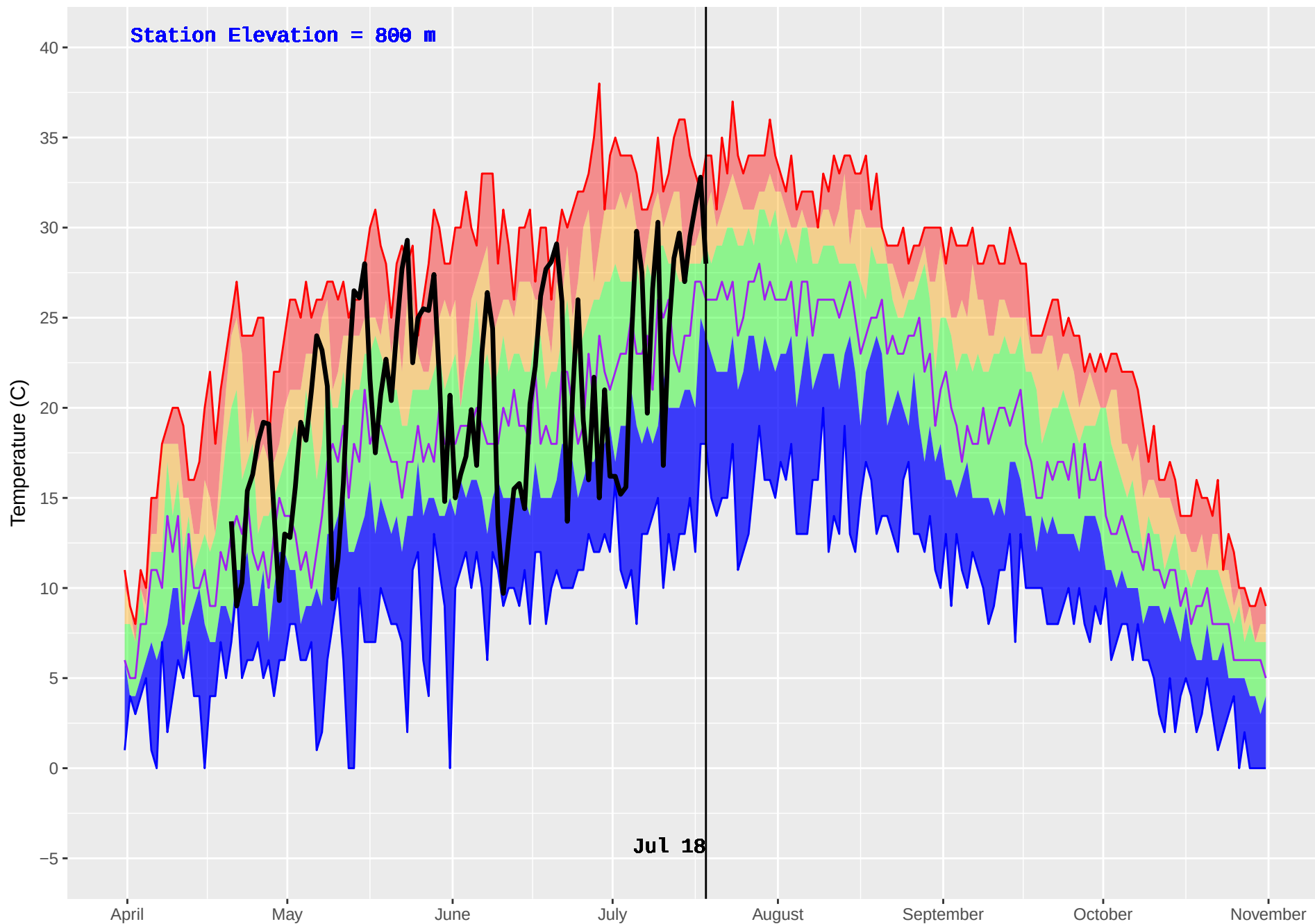
GOLD HILL (379) : Historical (1979–2016) and Current (2018) Daily Temperature
