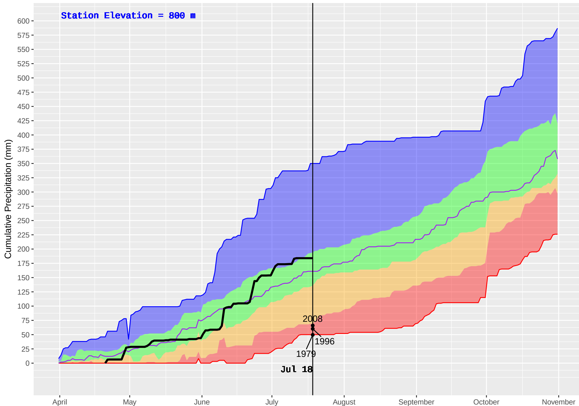
GOLD HILL (379) : Historical (1979–2016) and Current (2018) Daily Cumulative Precipitation
