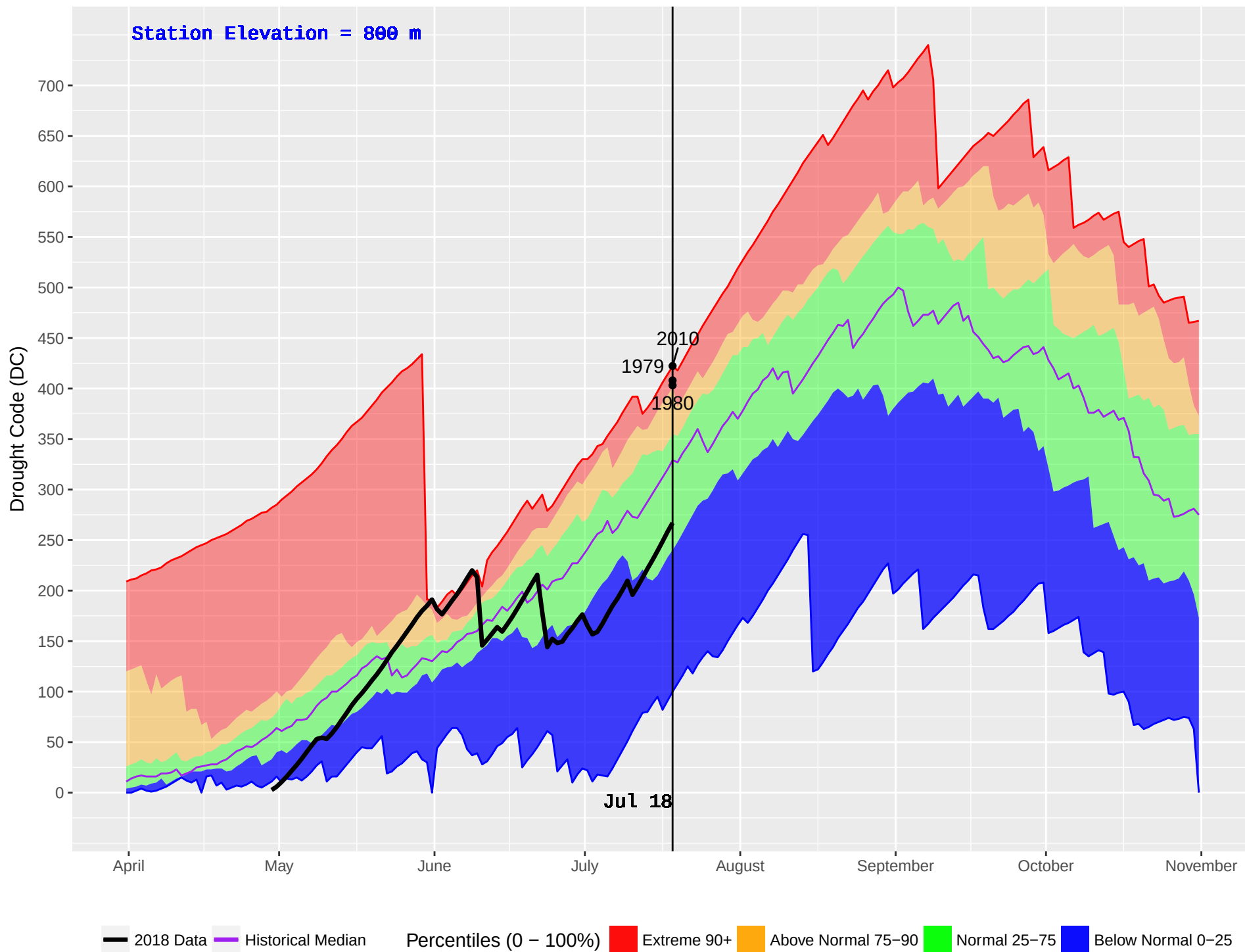
GOLD HILL (379) : Historical (1979–2016) and Current (2018) Daily Drought Code (DC)
