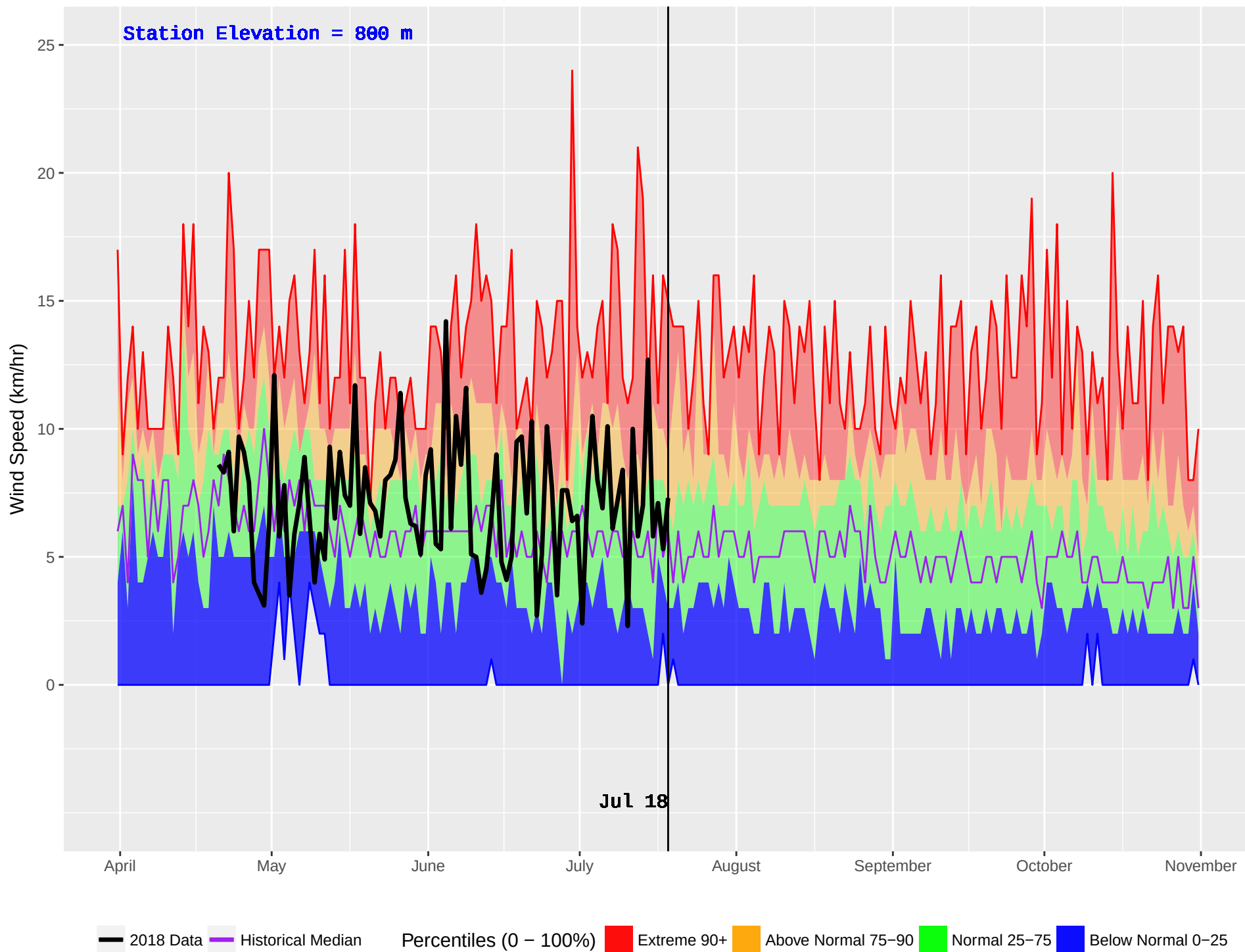
GOLD HILL (379) : Historical (1979–2016) and Current (2018) Daily Wind Speed
